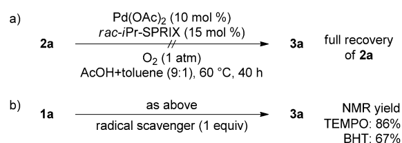
Scheme 5. Control experiments.
