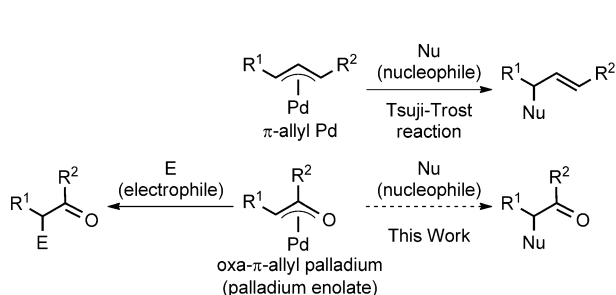
Scheme 1. General reactivity of \pi -allyl palladium complexes and oxa- \pi -allyl palladium complexes (palladium enolates).
